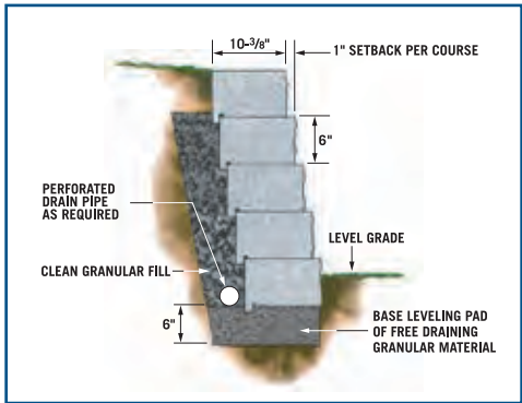
LEGACY STONE cross section
