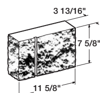
4" x 8" x 12"— Split Face Corner Single Grid
