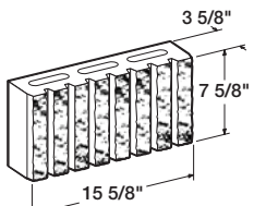
4" x 8" x 16"— Fluted Block - 8 Flute
