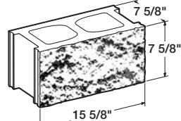
8" x 8" x 16"— Split Face
