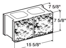
8" x 8" x 16"— Split Face Single Grid
