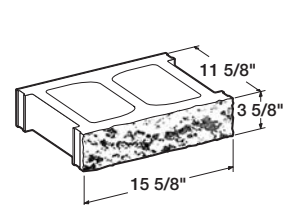
12" x 4" x 16"— Split Face Half Height
