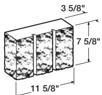
4" x 8" x 12"— Fluted Corner - 4 Flute Used with 4", 8" & 12" 4-Flute block
