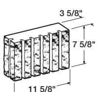
4" x 8" x 12"— Fluted Corner - 8 Flute Used with 4", 8" & 12"
