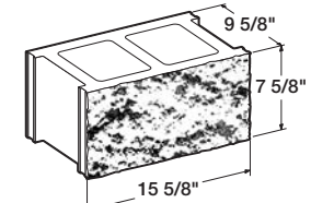
10" x 8" x 16"— Split Face
