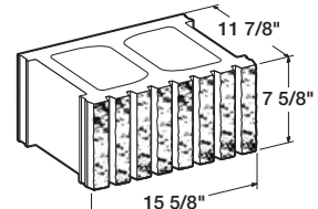
12" x 8" x 16"— Fluted Block - 8 Flute
