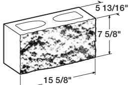
6" x 8" x 16"— Split Face
