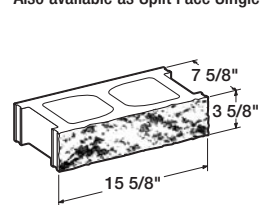
8" x 4" x 16"— Split Face Half Height
