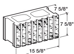
8" x 8" x 16"— Fluted Block - 8 Flute
