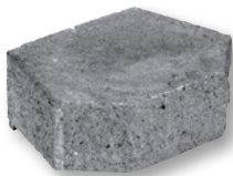
Garden Wall Three Plane Split Face 9" D, 4" H, 12" W Weight: 28 lbs *Total SFF x 3
